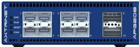
Status LEDs 10GbE/1GbE Ports 40GbE Ports
